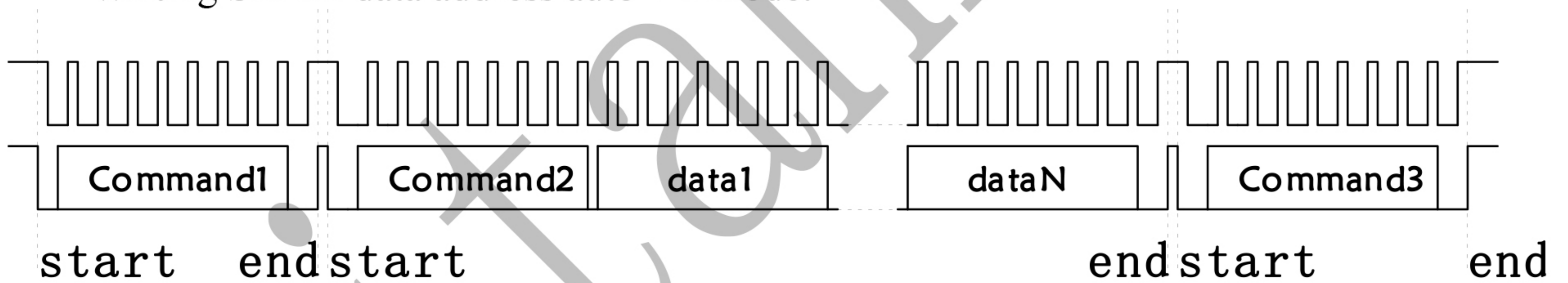
Figure 3: Format of auto address writing data
