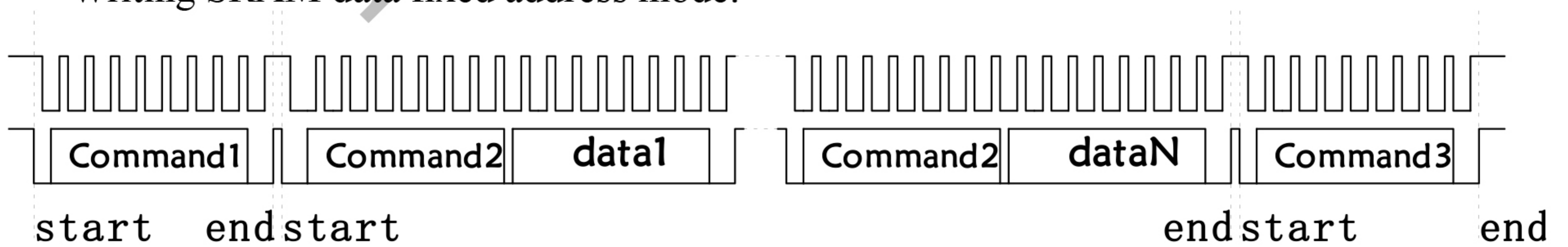
Figure 4: Format of fixed address writing data
