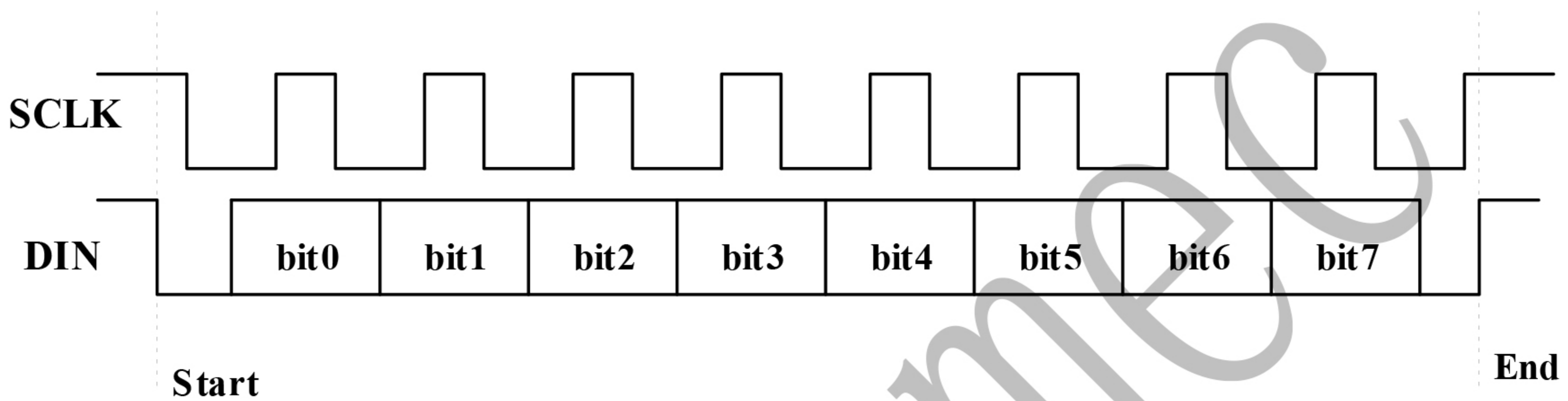
Figure 2: Command data transmission format
