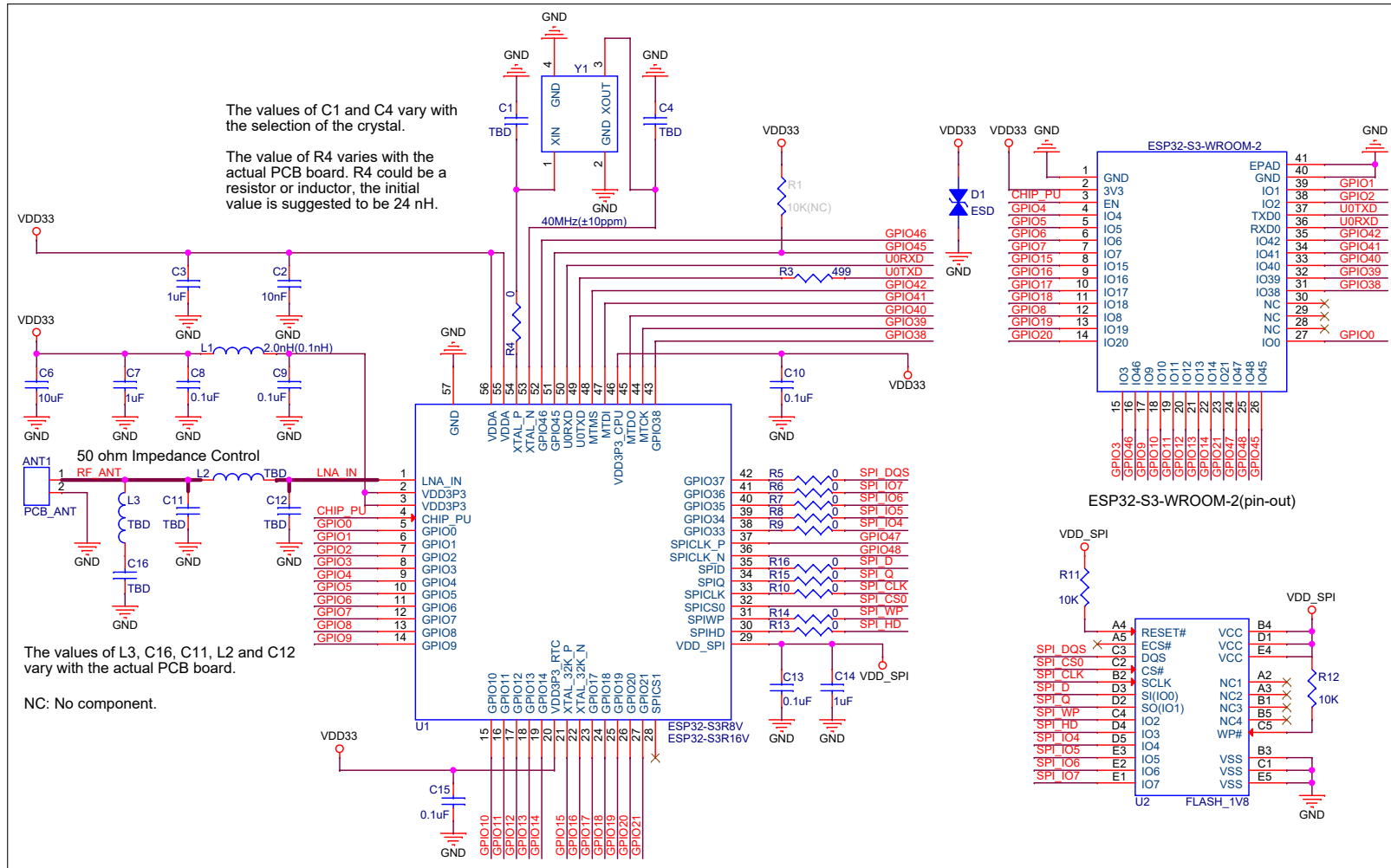
Figure 8-1. Schematics
