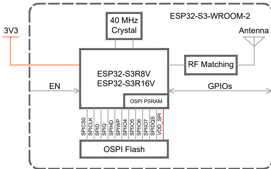
Figure 2-1. Block Diagram
