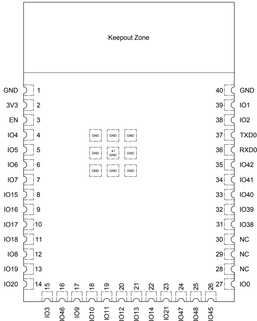
Figure 3-1. Pin Layout (Top View)
