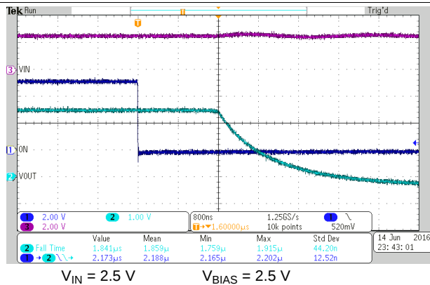
Figure 25. Turnoff Response Time
