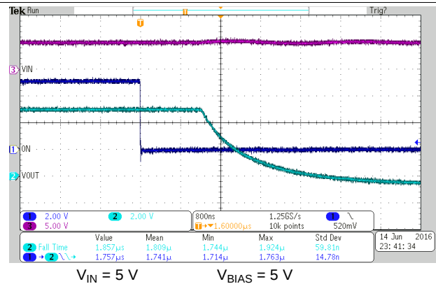
Figure 26. Turnoff Response Time
