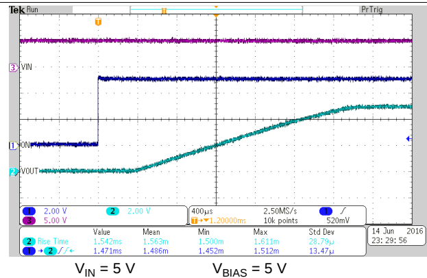
Figure 24. Turnon Response Time
