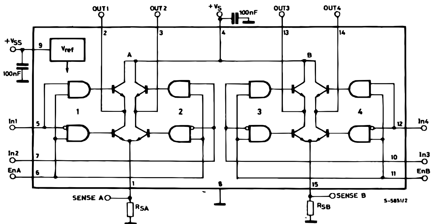
Figure 1. Block diagram
